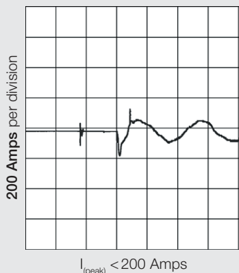
Fig. 3: With Series Reactor & With Pre-Charge Resistor
